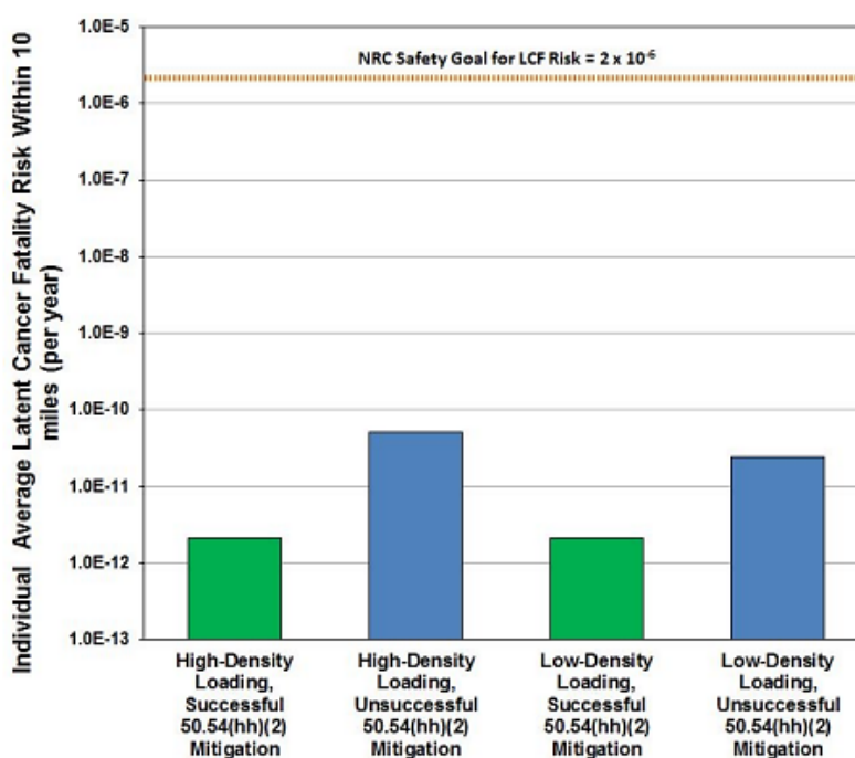
Figure E.3-5 Comparison of Population-Weighted Average Individual Latent Cancer Fatality Risk Results from NUREG-2161 to the NRC Safety Goal. Source: NRC 2014a. 36
